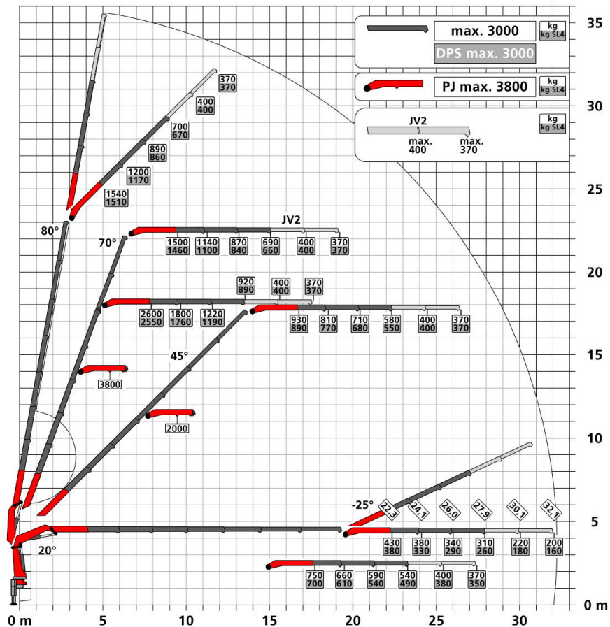
DPS-C Dual Power System
